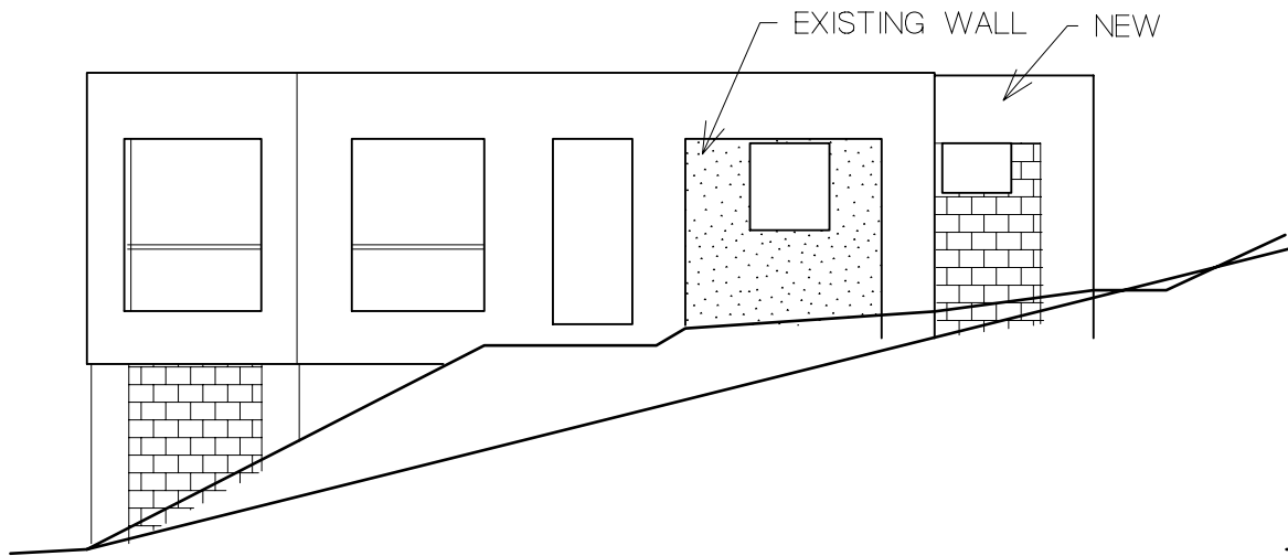
SOUTH ELEVATION
