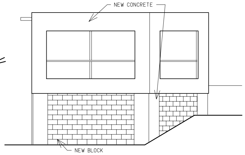
WEST ELEVATION
